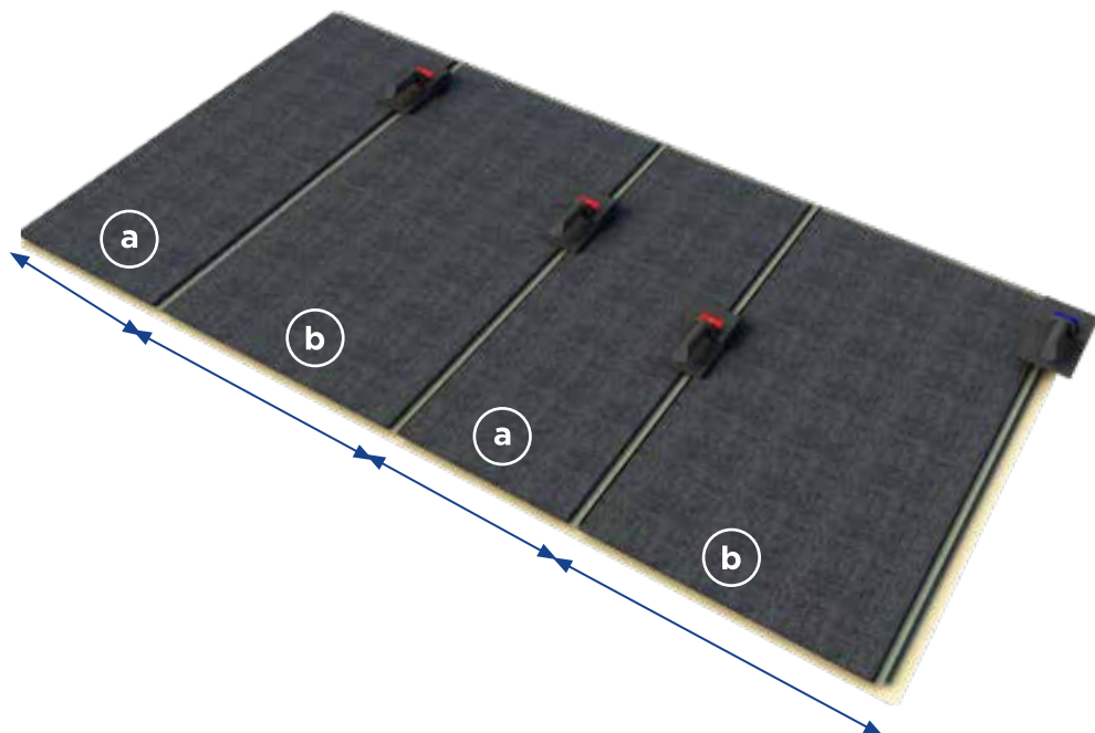
Half-lap joint cuts for forming a CLIMAVER® straight duct with the dimensions (a x b)
